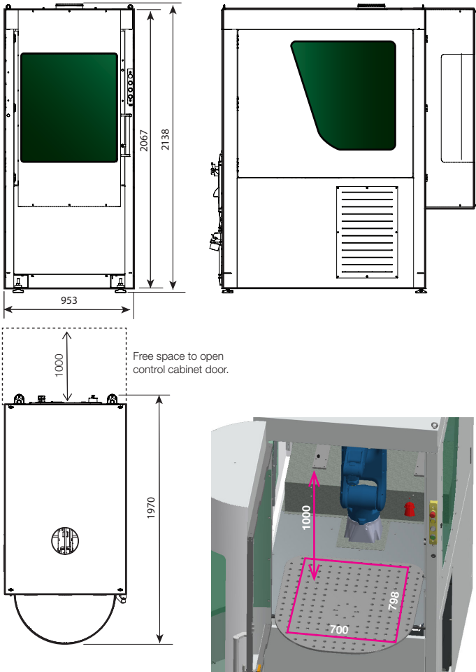
Fixture dimensions: 700x798x1000 mm (WxDxH).
