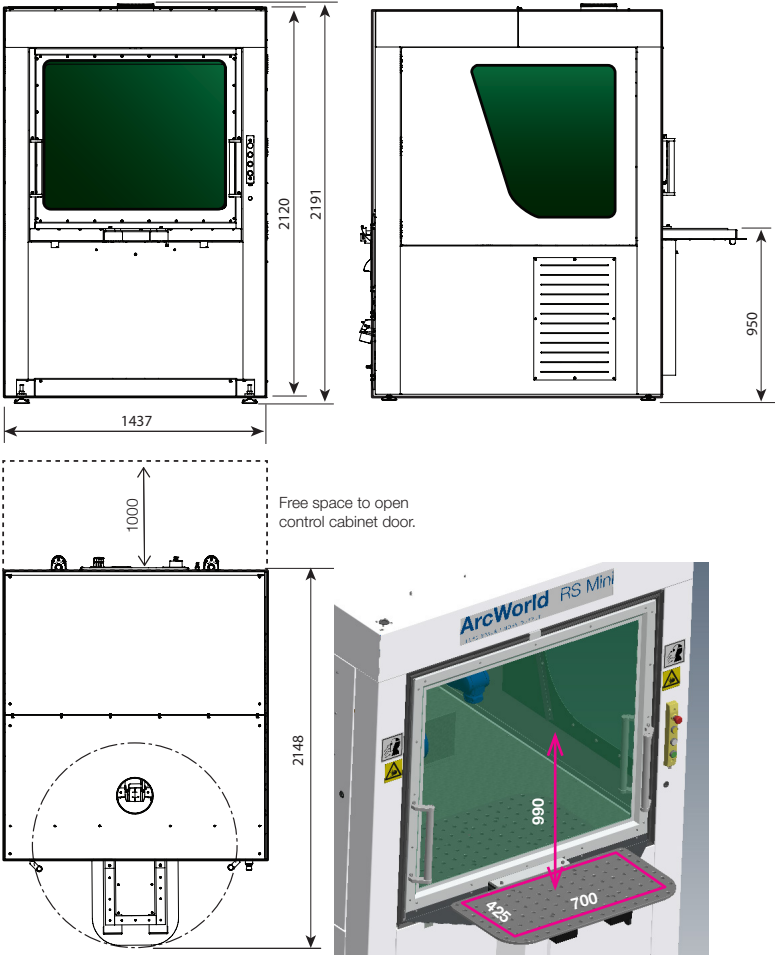
Fixture dimensions: 700x425x990 mm (WxDxH)
