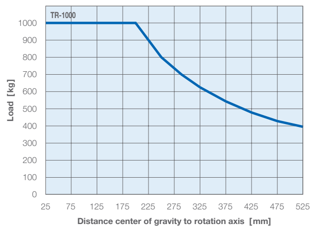
Load position – rotation-axis
