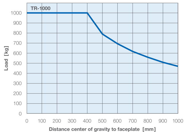
Load position – tilt-axis
