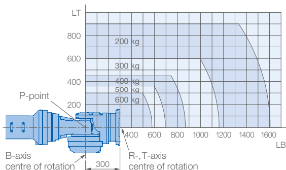
Allowable wrist load
