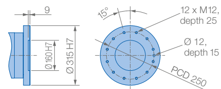
View A
