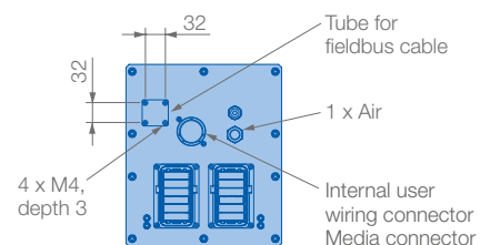
View B
