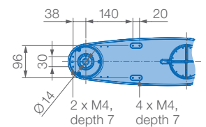
View E
