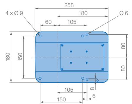
View C
